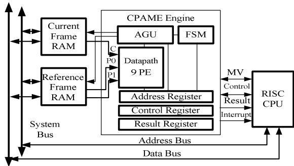
Fig. 5. Top level architecture of motion estimation
