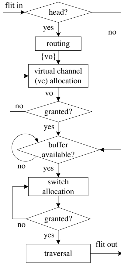
Fig. 3. Flow of a flit through routing, virtual channel allocation, switch allocation and switch traversal in a virtual-channel router [8]
