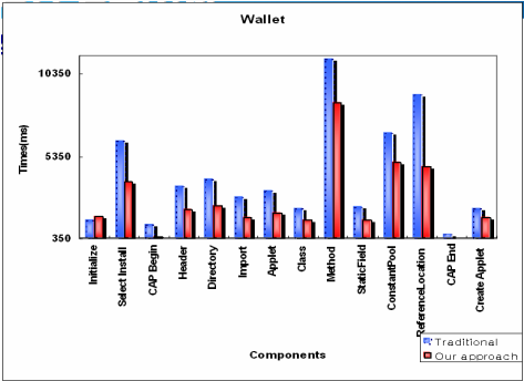
Fig. 15. The comparison between a traditional Java Card and our changed Java Card in regard to Wallet applet’s downloading and execution speed per each component
