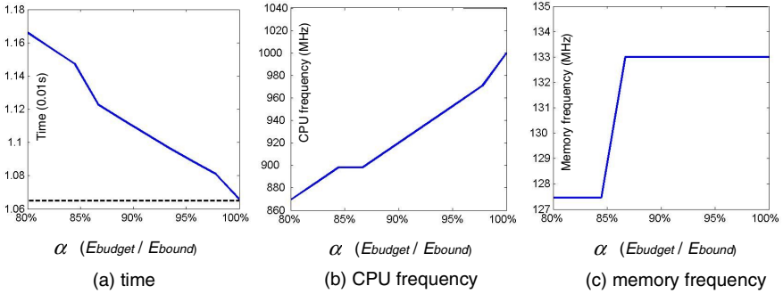
Fig. 10. The impact of E_{budget} on the optimization results when memory-bound case. C_c=1000 , C_m=150
