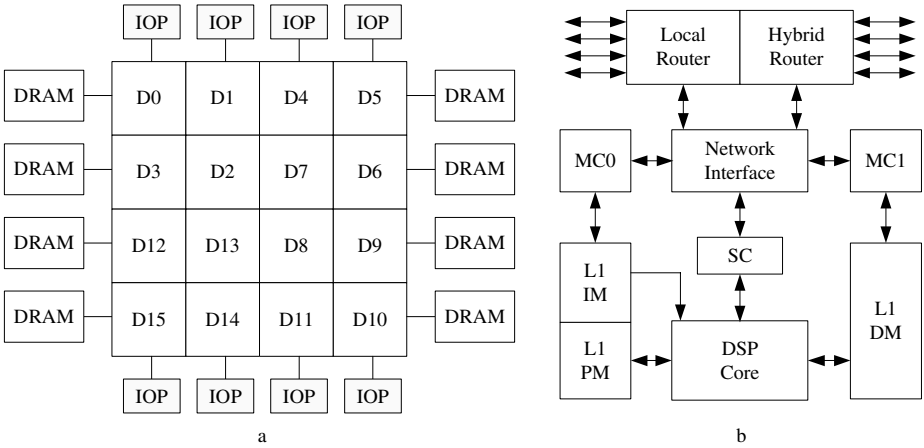
Fig. 1. DragonFly DSP architecture (a) and DragonFly DSP node (b)
