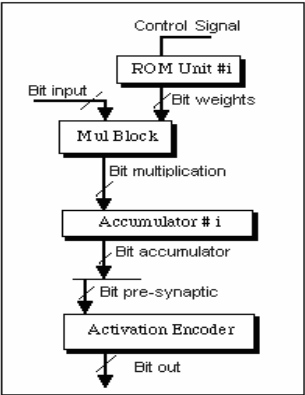
Fig. 4. The neuron architecture in the hardware approach
