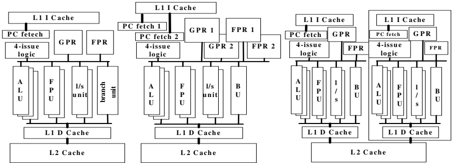
Fig. 1. ST superscalar, SMT and CMP architecture overview
