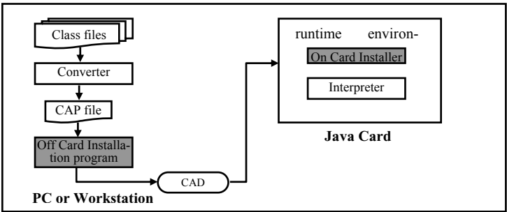
Fig. 2. Java Card Installer and off-card installation program [3]
