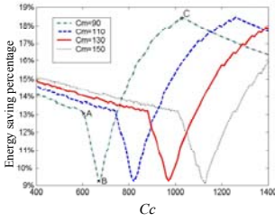
Fig. 3. Energy saving percentage as C_c and C_m vary
