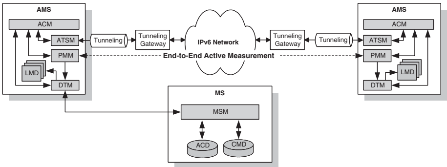
Fig. 1. Architecture of AMT6
