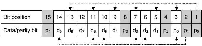
Fig. 2. Hamming code data and parity bits
