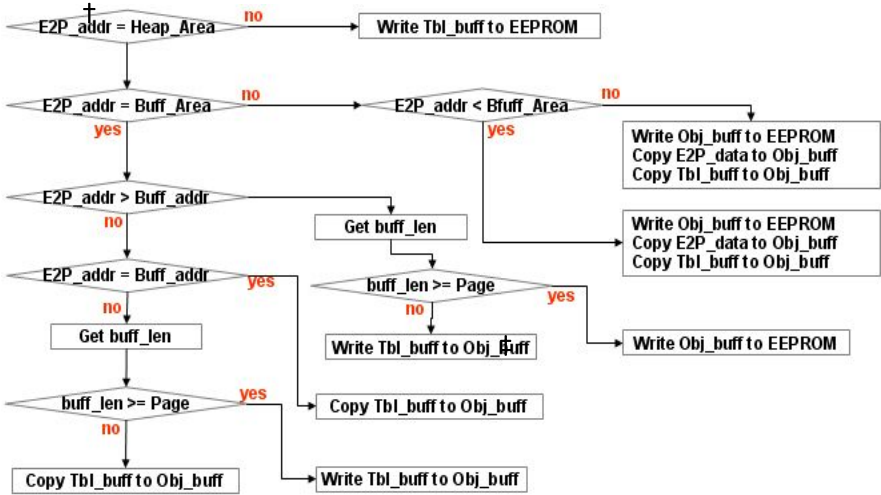
Fig. 12. The Object-buffer algorithm that checks continually the Min and Max points to write the object-buffer to EEPROM when Java Card writes data to heap area. ( \dagger E2p_addr : the EEPROM address that data will be written, \ddagger heap_buff(Obj_buff) : our new heap buffer with caching and buffering function for just heap area in EEPROM).
