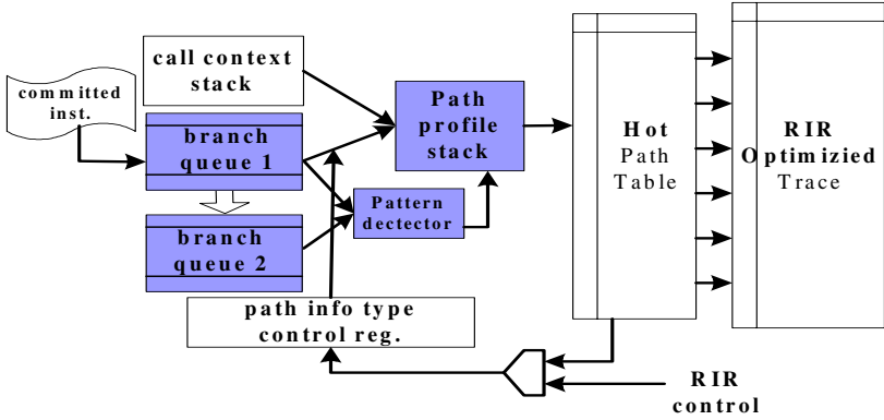
Fig. 3. Main hardware components in RIR
