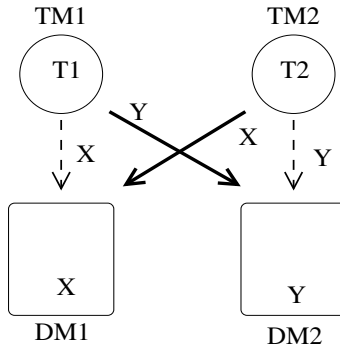
Fig. 3. Two system sites-case 2
