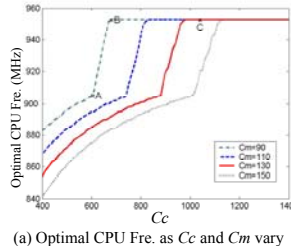
Fig. 4. Optimal CPU and memory frequencies as C_c and C_m vary
