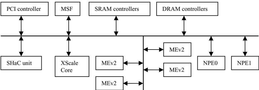
Fig. 1. Diagram of inner structure of IXP2350
