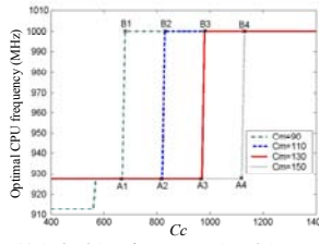
(a) Optimal CPU frequency as C_c and C_m vary
