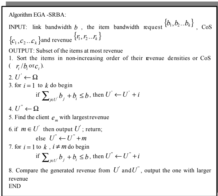
Fig. 2. Enhanced Greedy Algorithm for SRBA
