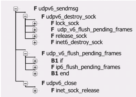
Fig. 6. Abstract view of Program 1
