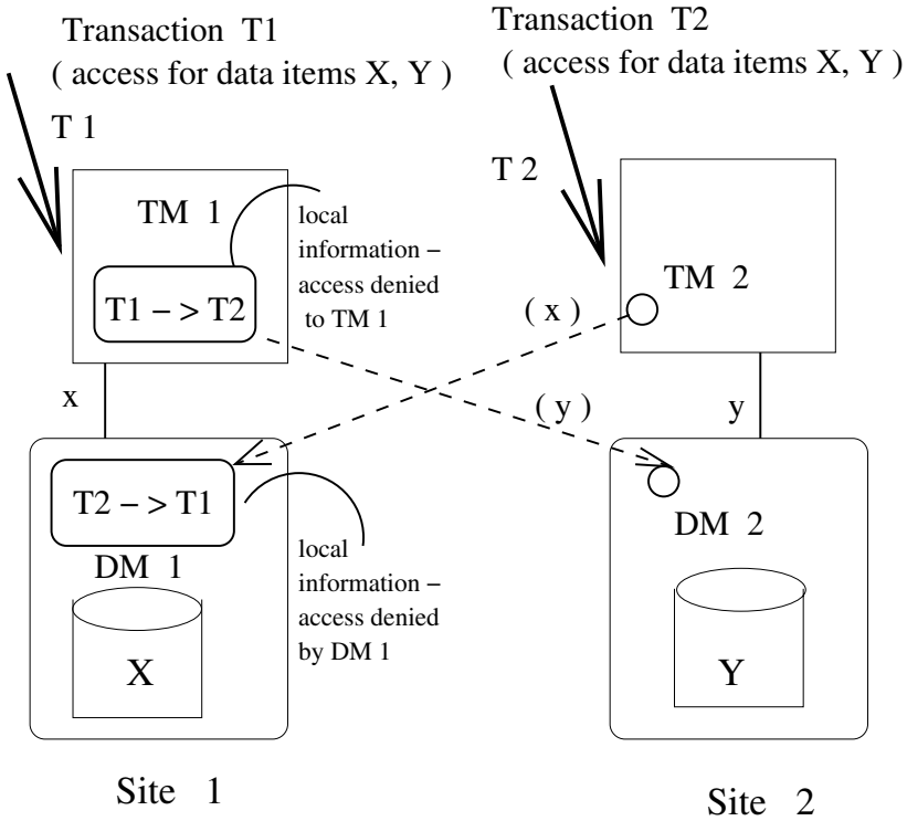
Fig. 2. Deadlock detection process with no inter-site messages
