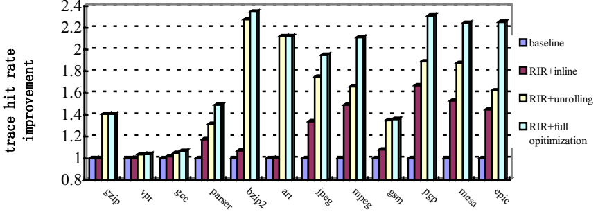
Fig. 10. Normalized trace hit rate for different policies
