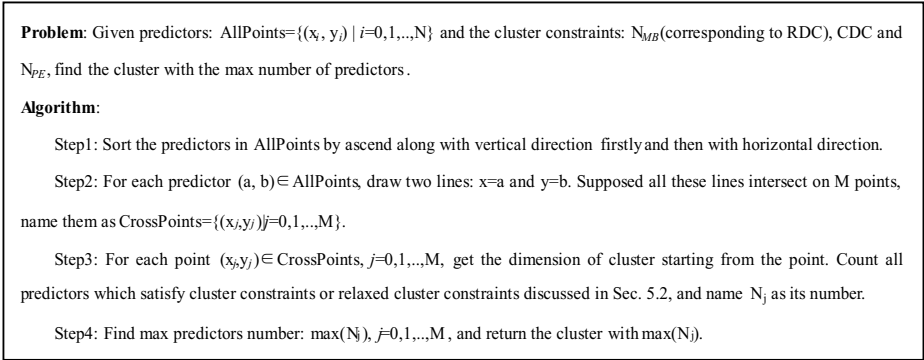
Fig. 7. Cluster partition algorithm
