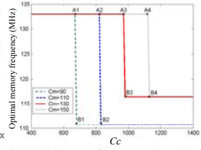
(b) Optimal memory frequency as C_c and C_m vary
