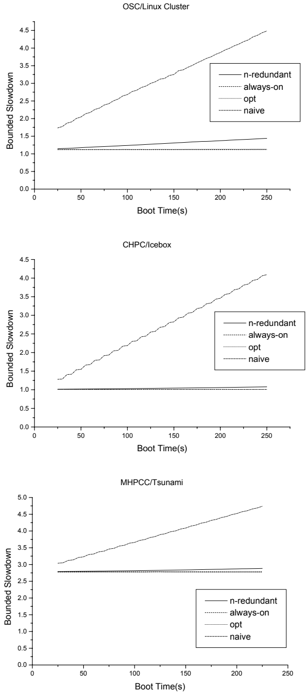
Fig. 3. Bounded-slowdown with different strategies
