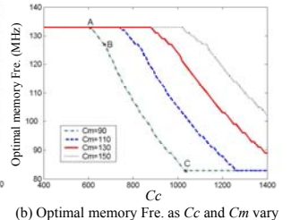
Fig. 4. Optimal CPU and memory frequencies as C_c and C_m vary
