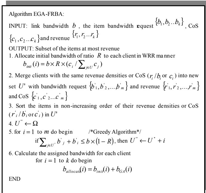
Fig. 3. Enhanced Greedy Algorithm for FRBA
