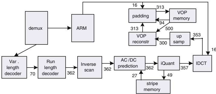
Fig. 1. Block Diagram of Video Object Plane Decoder (VOPD)
