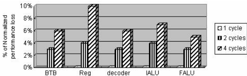
Fig. 5. The impact unideal power gating on performance
